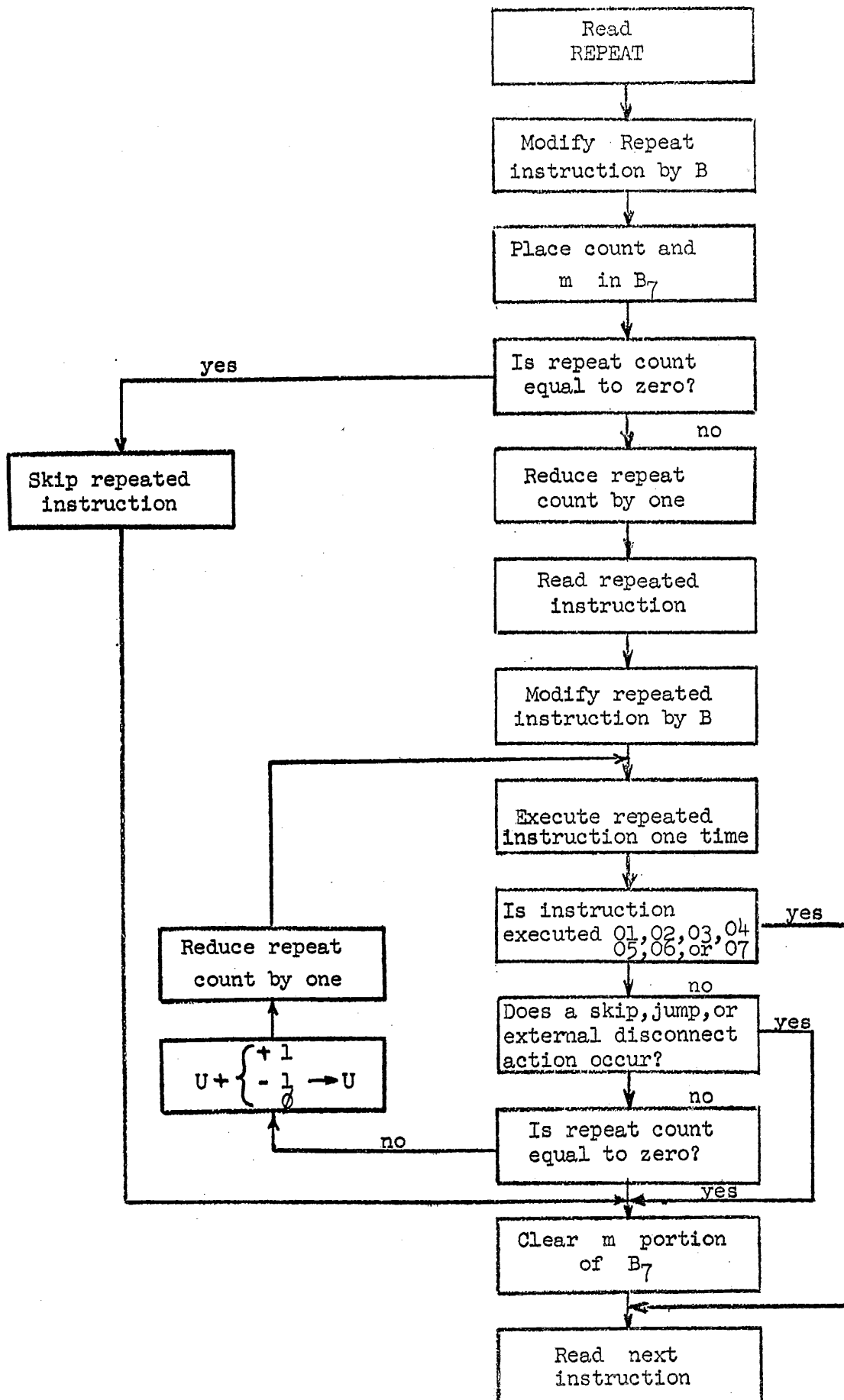
Figure 2 - Sequence of Operations for a Repeated Instruction
